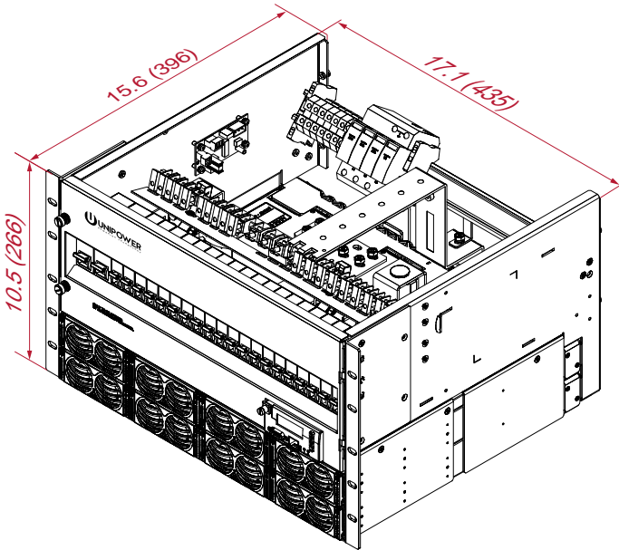
WITHOUT REAR COVER
