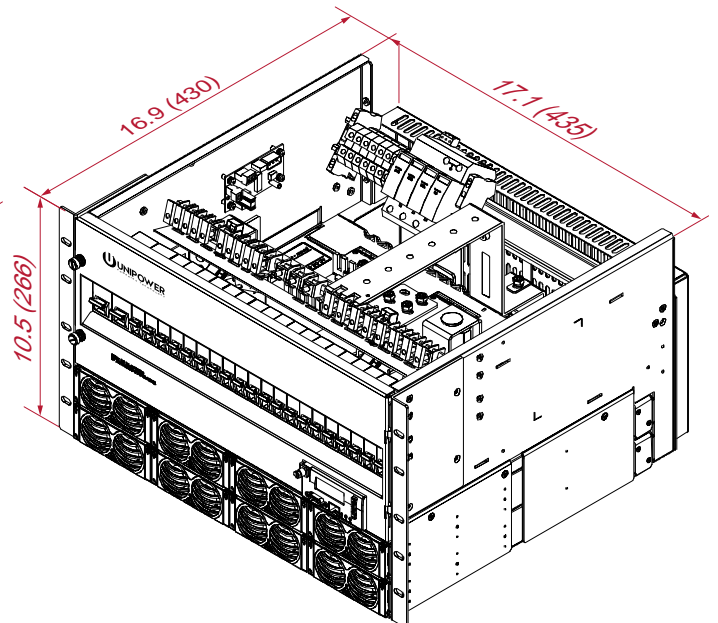
WITH REAR COVER
